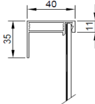
Detail C
